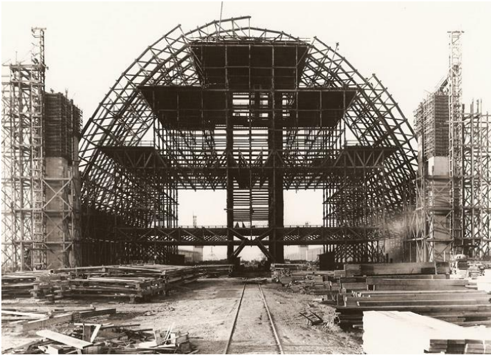
Hangar under construction with construction crew scaffolding. One of two completed hangars.
